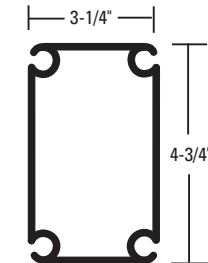
BEAM CROSS SECTION
